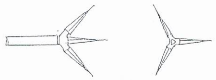
DETAIL LIGHTNING CONDUCTOR
